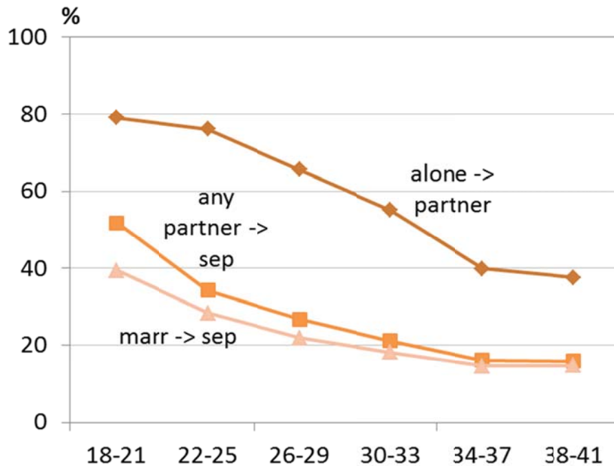
Figure 4: Proportion of women experiencing a change in their partnership status within 10 years, by initial age and state. Women aged 18-44. GB, GHS 2000-2005/7.
